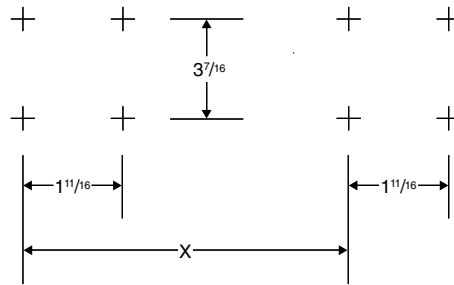
MOUNTING HOLE LOCATION DIAGRAM (Single Section Unit)
